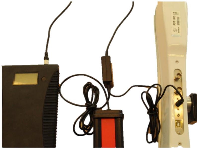
Figure 2. Battery pack connected to MFPA & IRIS camera
